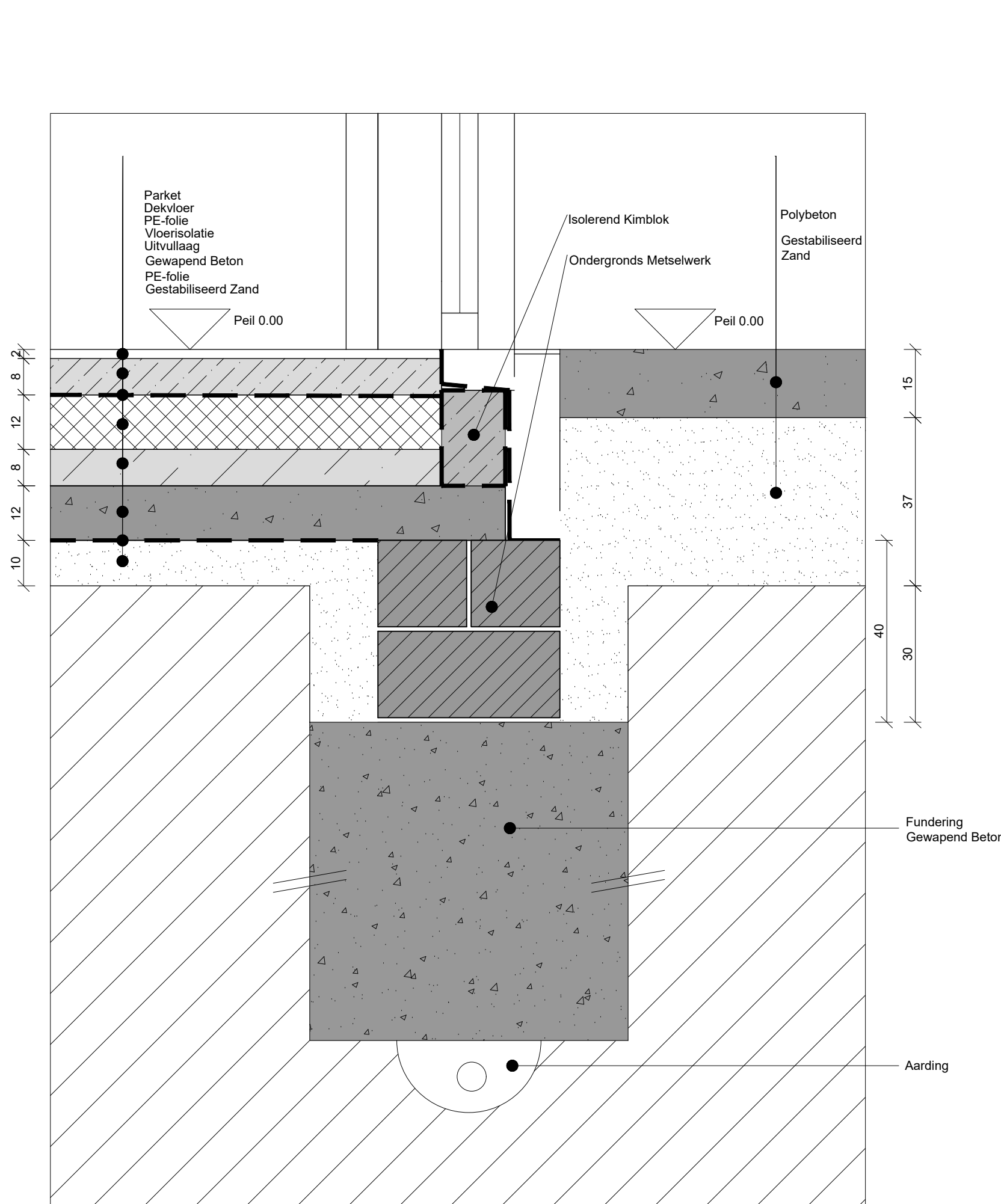
Detail 3 1/10
