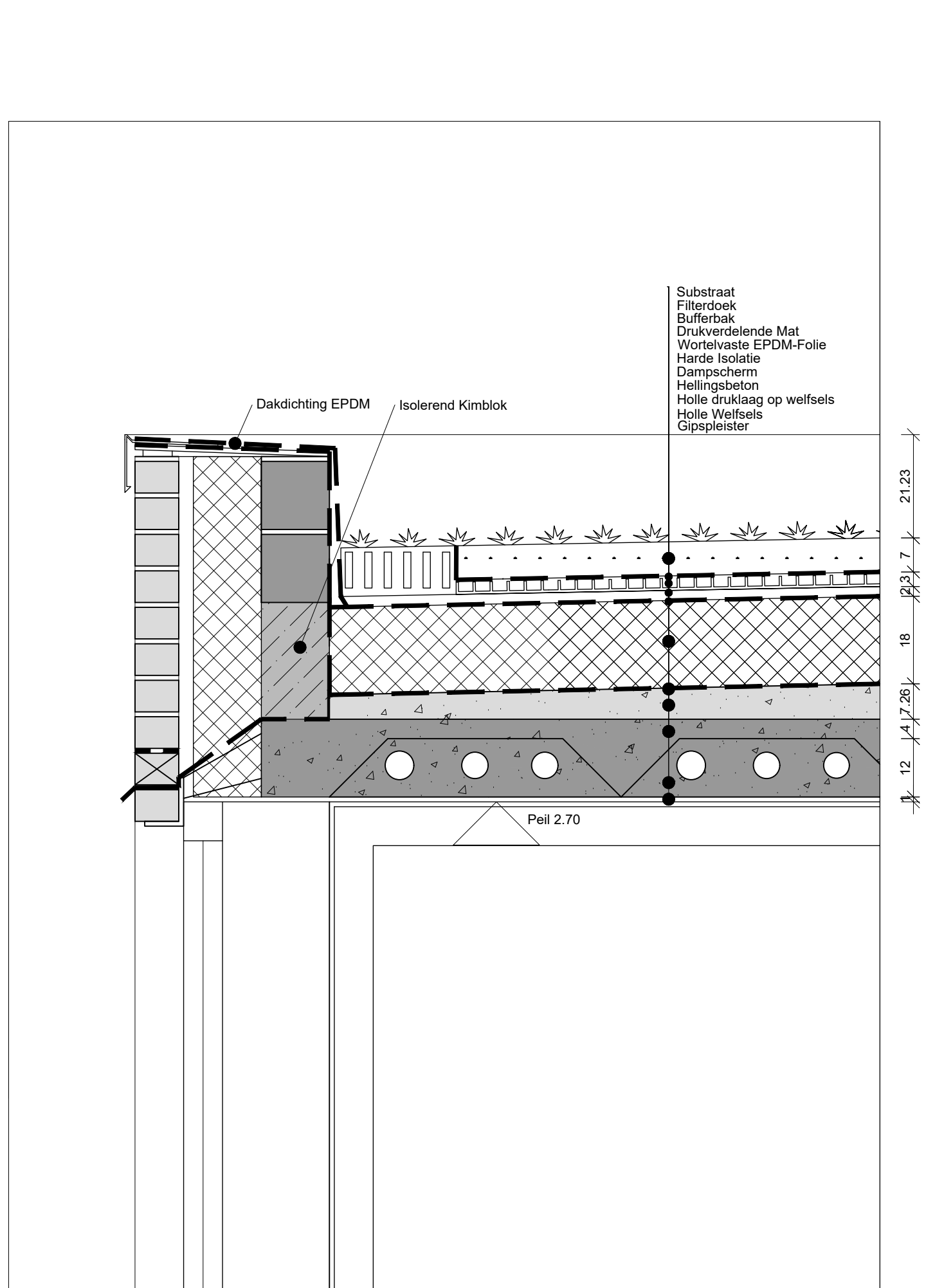
Detail 1 1/10
