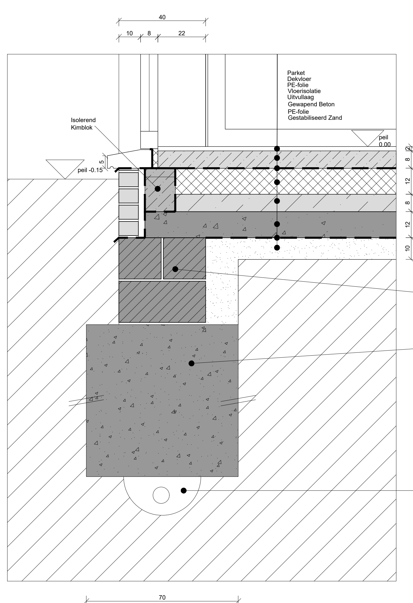
Detail 2 1/10
