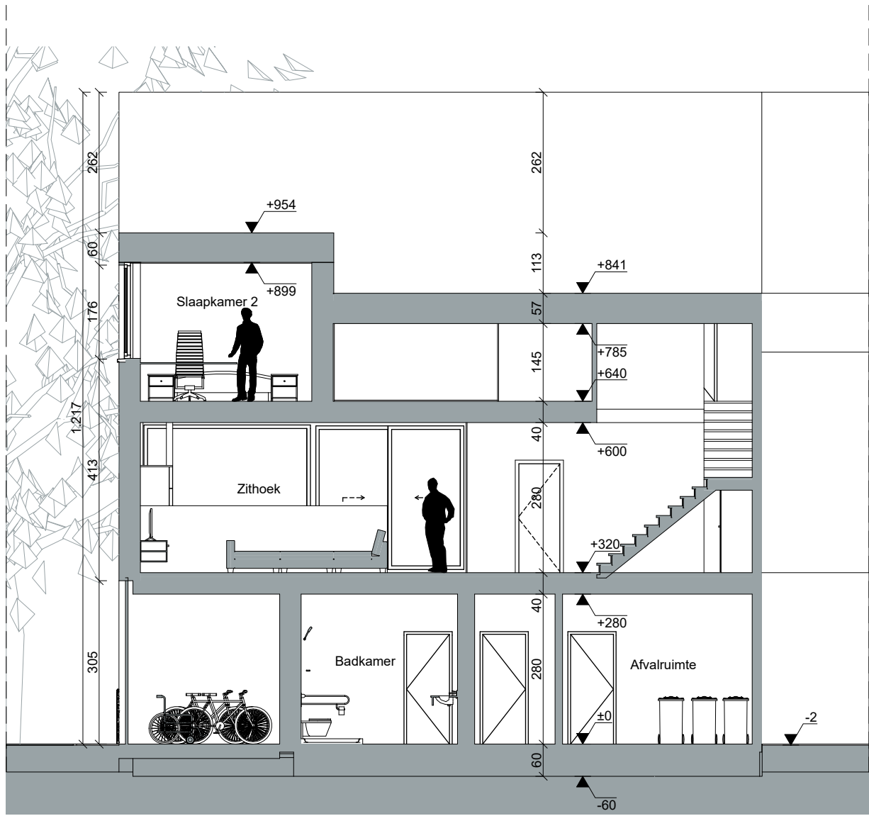
Sneede CC'
